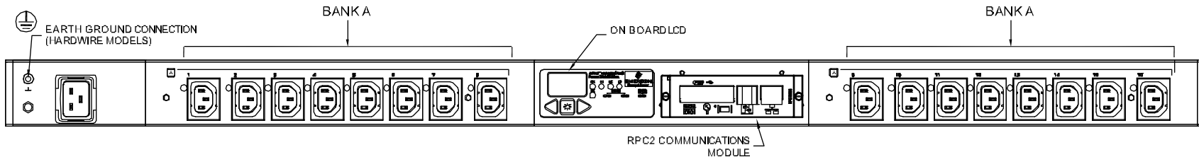
FRONT VIEW
