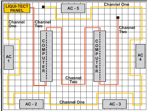
Liebert Leak Detection Systems can be configured to match the protection needs of any site.
